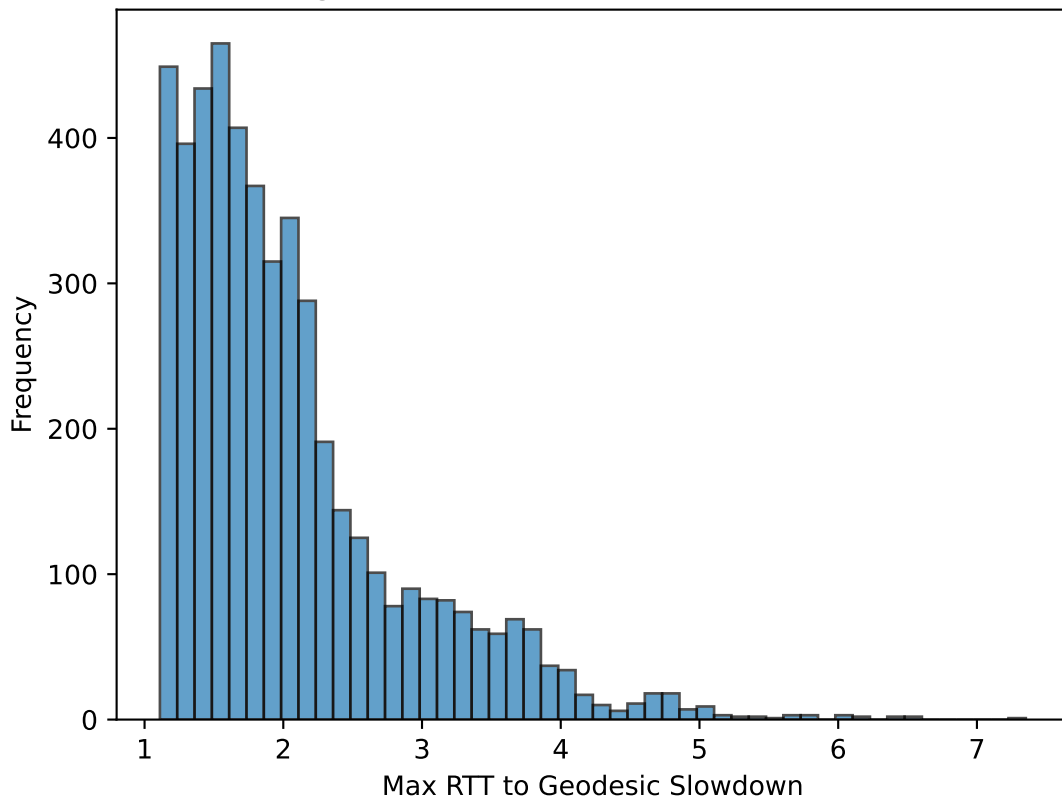
Histogram of Max RTT to Geodesic Slowdown
